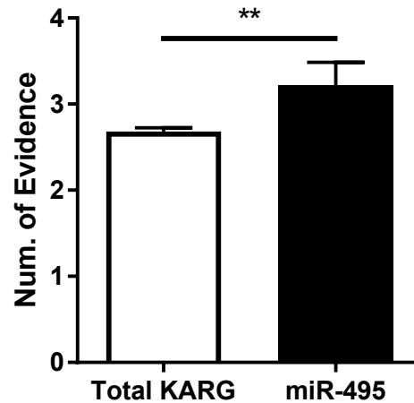
Fig AC.1. Predicted miR-495 targets from the KARG have more evidence for their involvement in addiction than the total KARG. The entire mouse KARG dataset was searched for miR-495 targets as in Fig. 1A, B and Table S1. Each gene in the dataset included a score for how many pieces of evidence linked the gene to addiction. Average evidence scores from the entire dataset in comparison to predicted miR-495 targets were compared. Mann-Whitney U, ** p < 0.01 .
